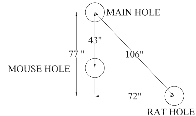
RATHOLE, MOUSEHOLE CONFIGURATION
